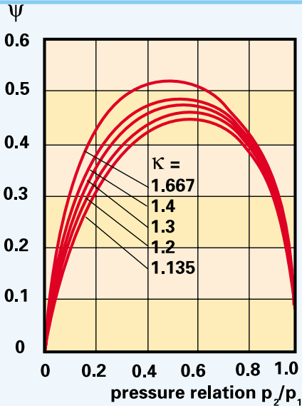
Flow coefficients as a function of the pressure relation for different \kappa -values.
